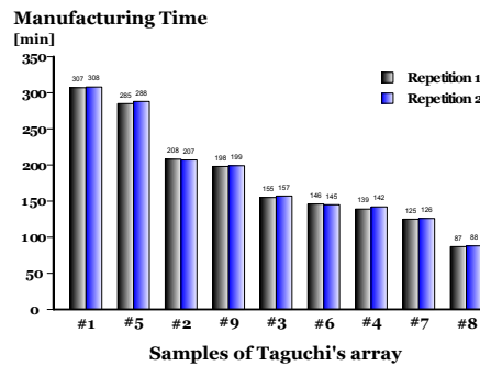
Figure 6: Fabrication time of the control factor sorted in descending order
