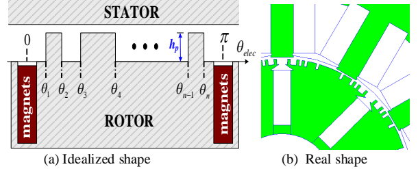
Fig. 2. Principle of grooved rotor with inset Permanent Magnets.
