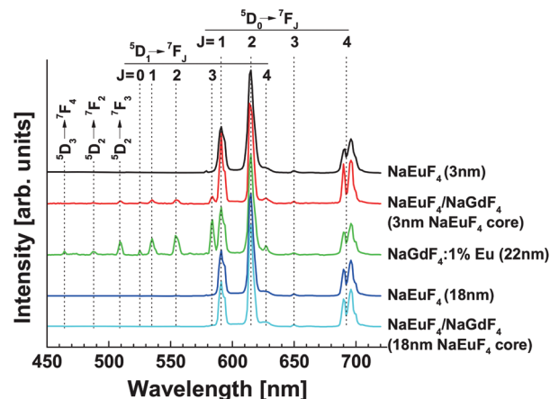
Fig. 5 Normalized emission spectra of 3 nm \beta -NaEuF 4 , 20 nm \beta -NaEuF 4 /NaGdF 4 NPs with a 3 nm \beta -NaEuF 4 core, 22 nm \beta -NaGdF 4 NP doped with 1% Eu, 18 nm \beta -NaEuF 4 and 22 nm \beta -NaEuF 4 /NaGdF 4 NPs with an 18 nm \beta -NaEuF 4 core. The spectra were recorded under 394 nm excitation of the Eu 3+ ions ( ^7F_{0,1} \rightarrow ^5L_6 ). All particles consist of hexagonal phase ( \beta -phase).
