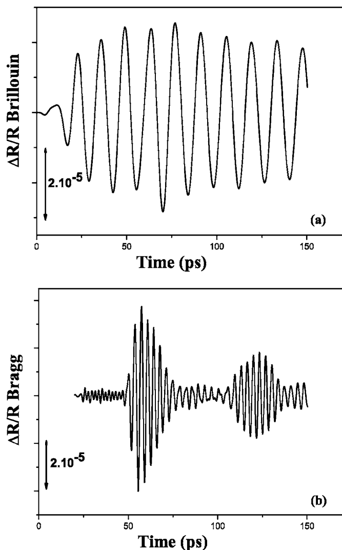
FIG. 5. (a) Brillouin oscillation and (b) Bragg reflection oscillation after Bessel numerical filtering of the curve in the inset of Fig. 3.
