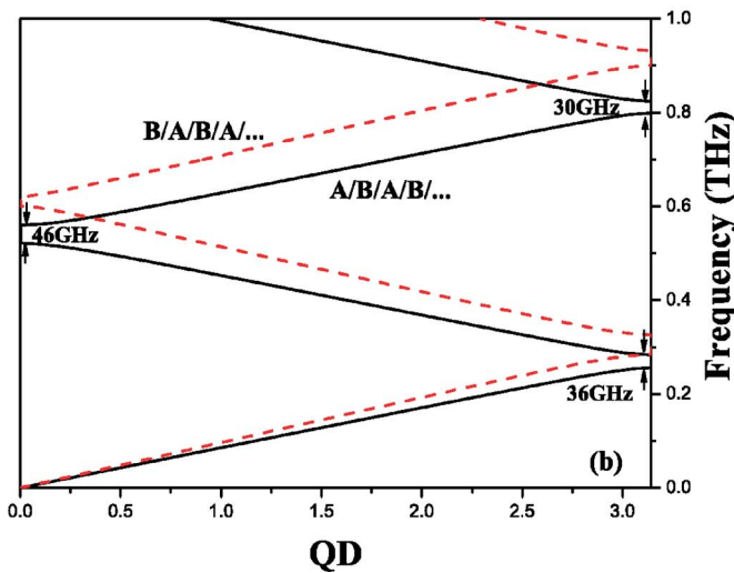
FIG. 2. (Color online) (a) Calculated phonon reflection rate for an A/B/A/B\dots configuration of the SL, and (b) phonon-dispersion relation for both A/B/A/B\dots and B/A/B/A\dots configurations of the SL, with A \equiv \text{Si}_{0.4}\text{Ge}_{0.6} and B \equiv \text{Si} .
