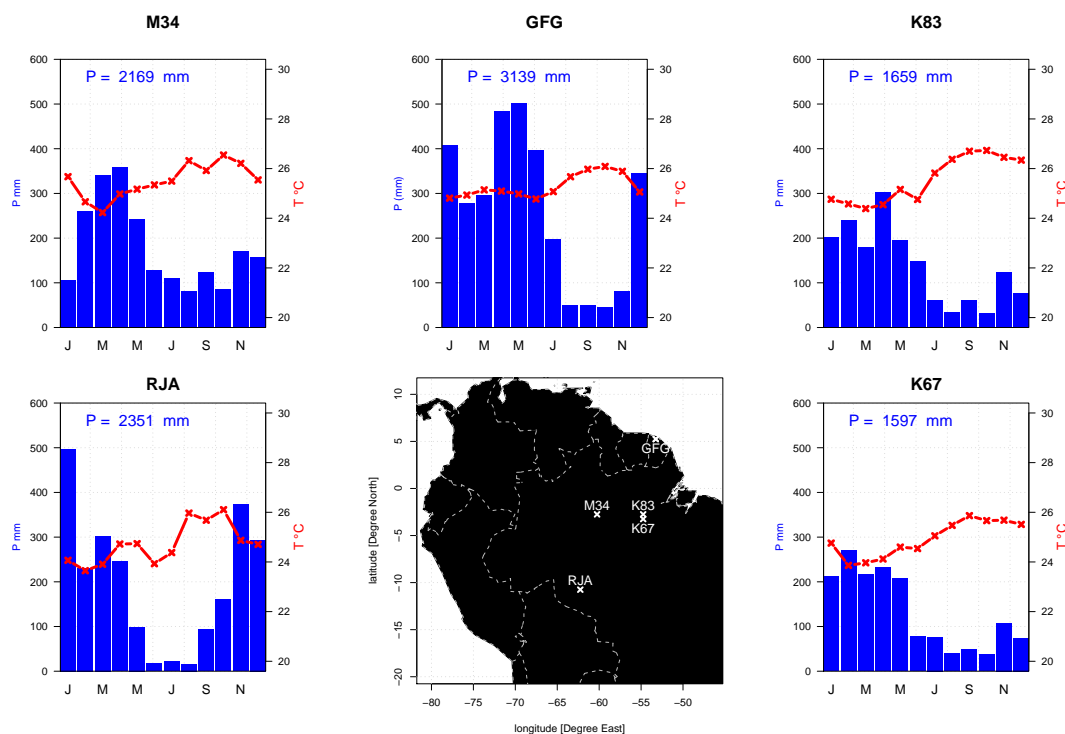
Figure 1. Mean annual cycle of precipitation (blue) and temperature (red) calculated over 3 years (see Table 1), and the location of the flux towers used in this study.
