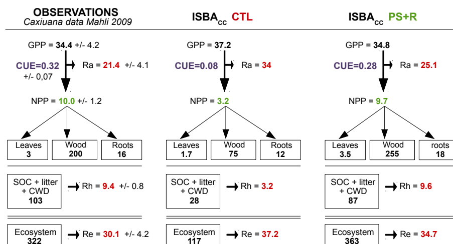
Figure 9. Annual carbon pools (in \text{tC ha}^{-1} ) and fluxes (in \text{tC ha}^{-1} \text{yr}^{-1} ) from a synthesis of observations at Caxiuanã (Malhi et al., 2009) compared to ISBA CC (CTL and PS+R simulations). Adapted from Randerson et al. (2009).
