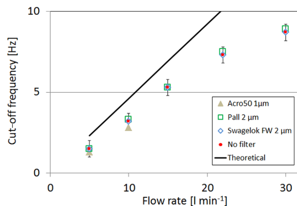
Figure 4. Cut-off frequencies (Hz) as a function of the flow rate (L min -1 ) for LI-7200 with ACRO 50 (grey triangle), PALL 2 µm (green squares), Swagelok FW 2 µm (blue diamonds), and without any filter (red dots). The full line corresponds to the theoretical prediction given by Eq. (2).
