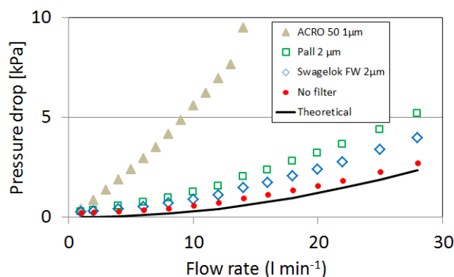
Figure 3. Pressure drop in the IRGA cell (kPa) as a function of the flow rate (L min -1 ) for different filters: ACRO 50 (triangles), PALL 2 µm (squares), Swagelok FW 2 µm (diamonds) and without any filter (dots). The theoretical curve (Eq. 1) is given by the continuous line.
