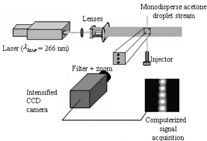
Fig. 3. Acetone PLIF experimental set-up.
