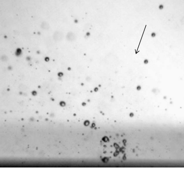
Fig. 6. Image illustrating the splashing regime ( T_w = 250 °C, D = 115 \mu m, V = 7.2 m/s, \alpha = 74^\circ , f = 10 kHz).
