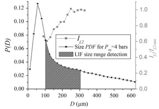
Fig. 9 Size range dynamic of LIF technique superimposed on the droplet size distribution for the spray (2) with P_{\text{inj}} = 4 bars. Evolution of the fluorescence intensity collected on the second spectral band as a function of the droplet diameter
