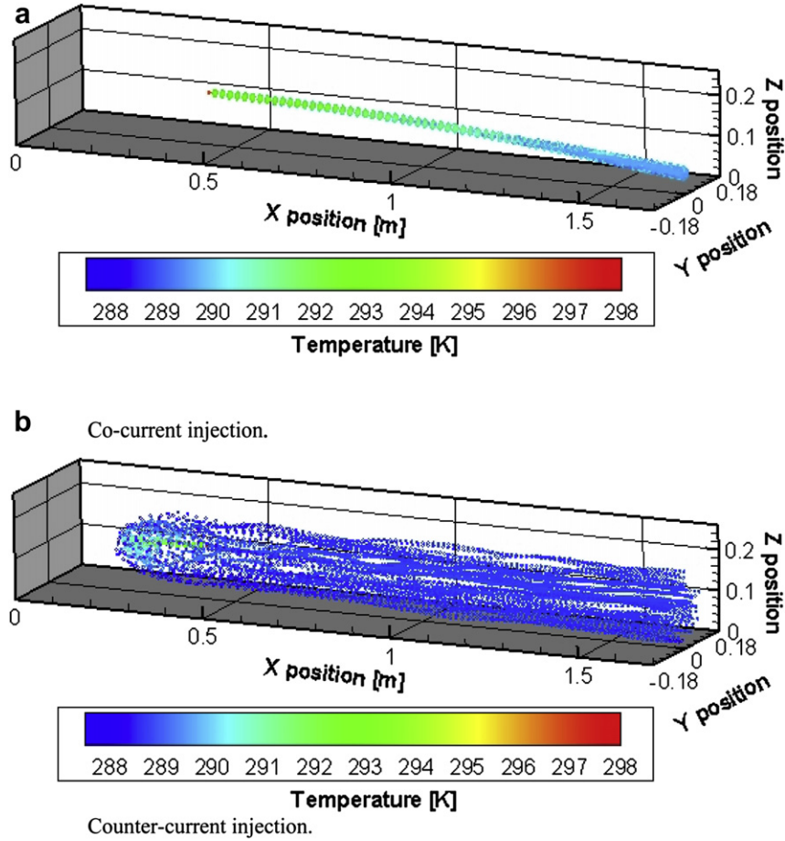
Fig. 2. Typical trajectories of 25 \mu\text{m} droplets in an air flow with average velocity of 1 m/s, from a preliminary academical study. Droplets are injected with initial velocity of 10 m/s in a cone with angle 72^\circ in co-current direction (Fig. 2a) and counter-current direction (Fig. 2b).
