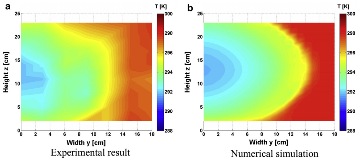
Fig. 5. Temperature distribution in the transverse section 5 cm downstream the nozzle injection. The C01 nozzle is used with a counter-current injection. The simulation is based on the code described in [7].
