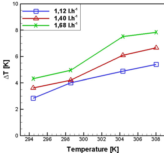
Fig. 6. Temperature cooling upstream the heat exchanger as a function of inlet air temperature: the difference is plotted between the average temperature at the inlet section of the channel and the temperature at the location of the exchanger, for three studied water flow rates.
