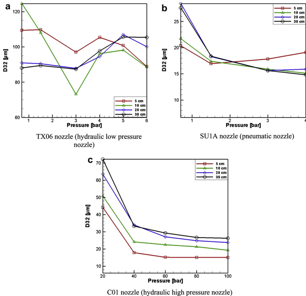
Fig. 3. Sauter mean diameter along the spray axis for the three nozzle types, as a function of feed pressure, for increasing distance below the injection point.
