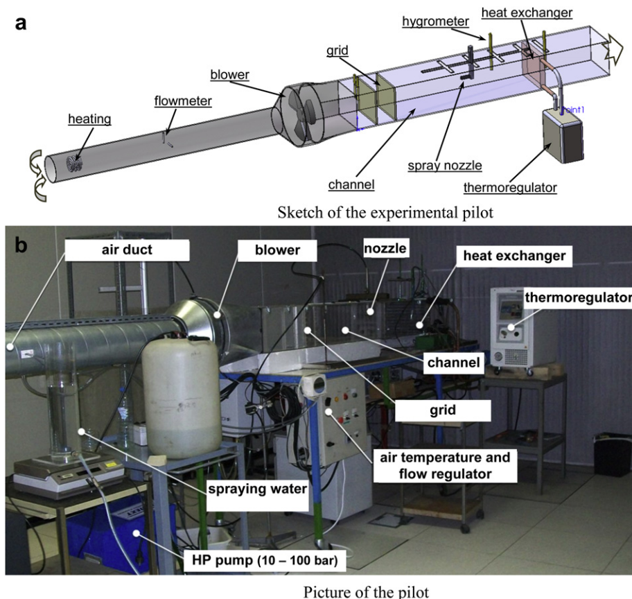
Fig. 1. Experimental setup.
