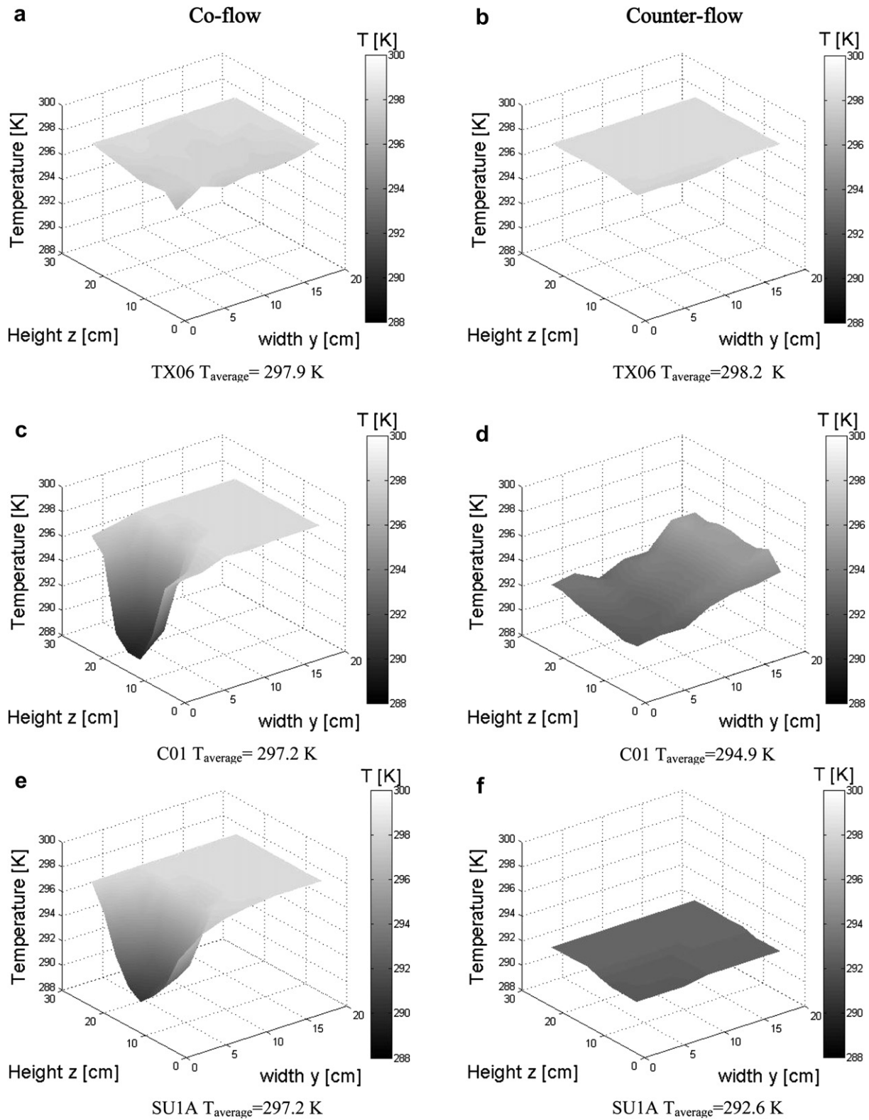
Fig. 4. Temperature distribution in a transverse section 40 cm downstream in the channel flow, for the three nozzle types, for co-current and counter-current injection of the spray. The average temperature in the section is indicated with the nozzle type.
