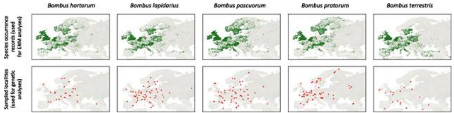
Figure 1. West Palaearctic maps with Bombus hortorum , B. lapidarius , B. pascuorum , B. pratorum and B. terrestris occurrence data used in ecological niche modelling analyses (above) and maps of sampling localities for which DNA sequence data (one mitochondrial and two nuclear loci) were available and analysed in this study.
