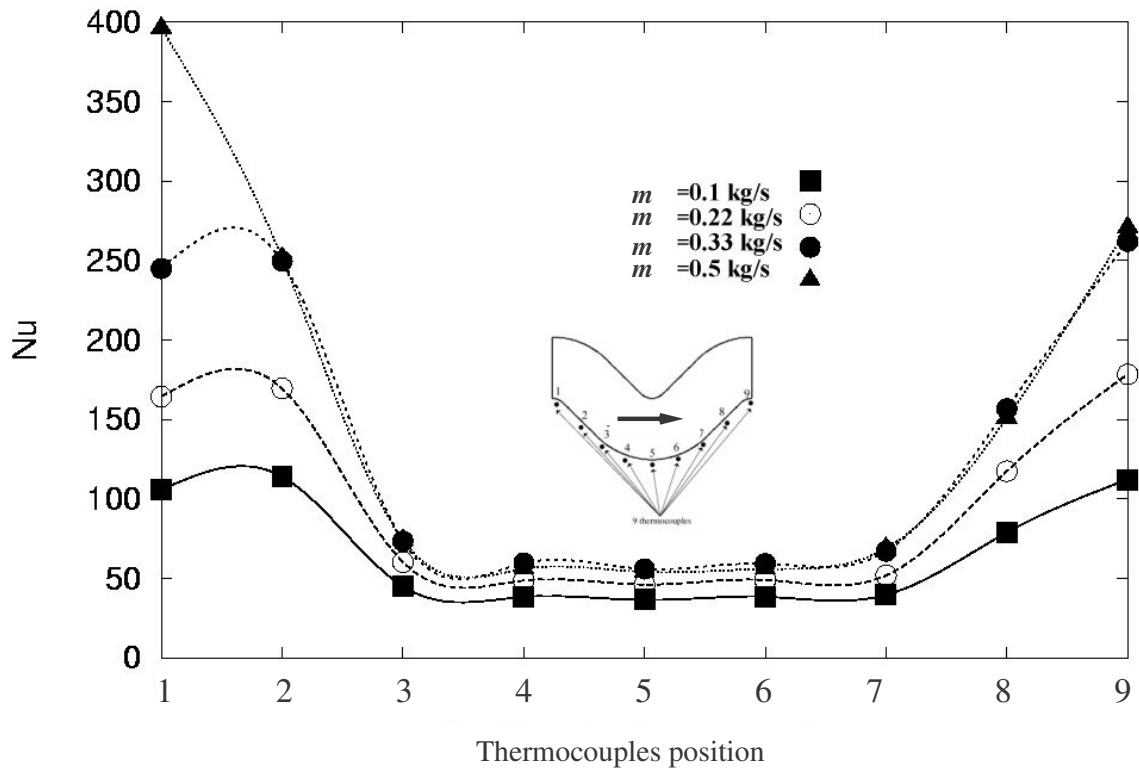
Fig. 9 – Evolution of the Nusselt number - T_{in} = 70^{\circ}C and Q = 56.9 \text{ kW} \cdot \text{m}^{-2}
