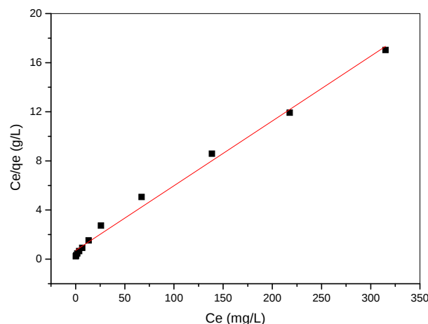
Figure 10. Langmuir isotherm plot for adsorption of \text{Ni}^{2+} on the maghnite. T = 293 K, initial pH 7.5, m/V = 10 g/L.
