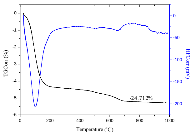
Figure 2. TG-DTA analyse of natural maghnite.
