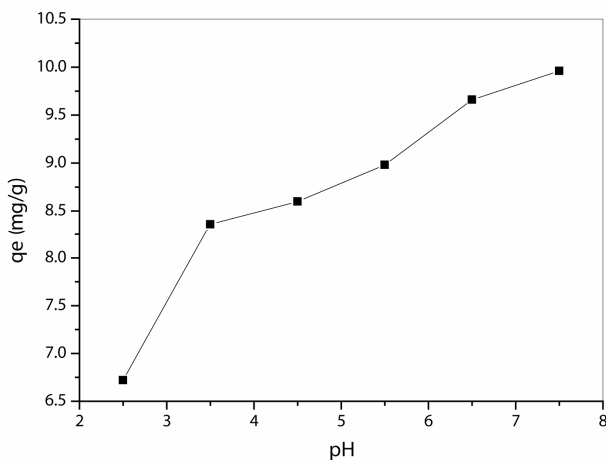
Figure 7. Effect of pH on adsorption capacity of maghnite for Ni(II).
