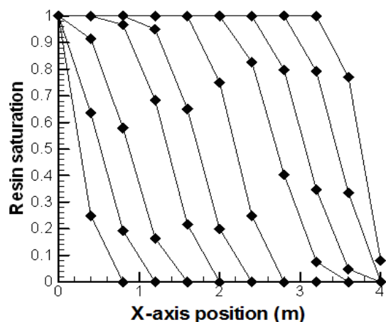
FIG. 10 RESIN SATURATION PROFILE AT DIFFERENT TIME
