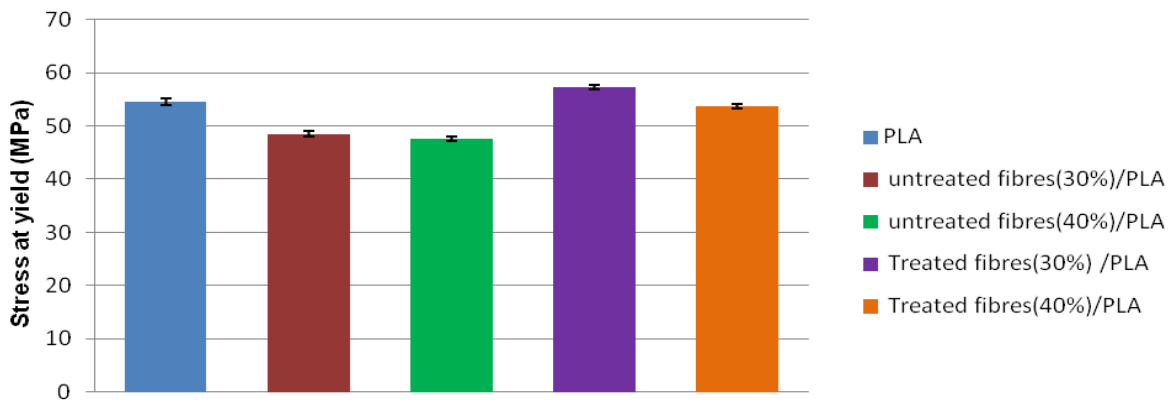
Figure 4. Stress at yield for composites materials with untreated and treated fibres.
