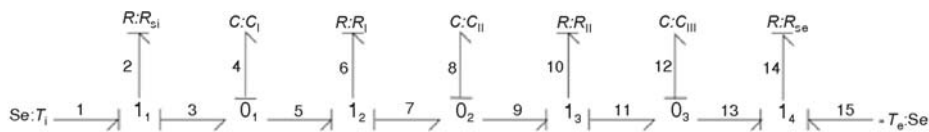
Figure 3. Numerated PBG model of the wall
