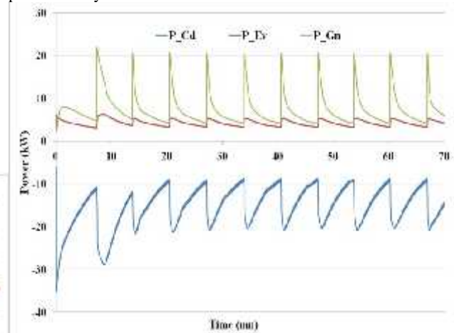
Figure 12 Thermal power dynamic behavior at the adsorbent beds, condenser, and evaporator (numerical values)
