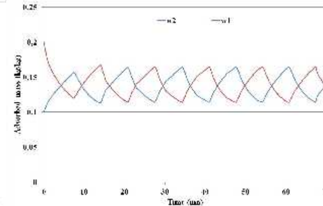
Figure 13 Adsorbed mass of water at the adsorbents (numerical values)
