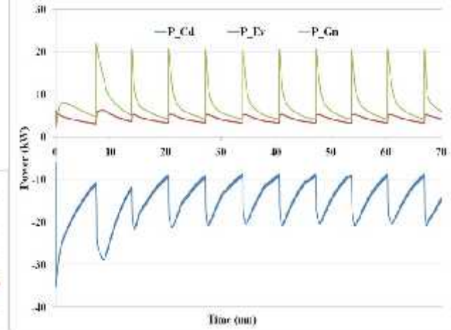
Figure 12 Thermal power dynamic behavior at the adsorbents, condenser, and evaporator (numerical values)
