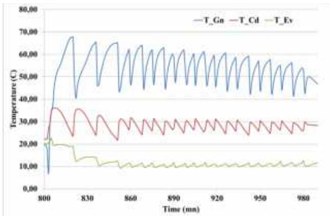
Figure 4 Evolution of the desorption, condensing and evaporation temperatures
