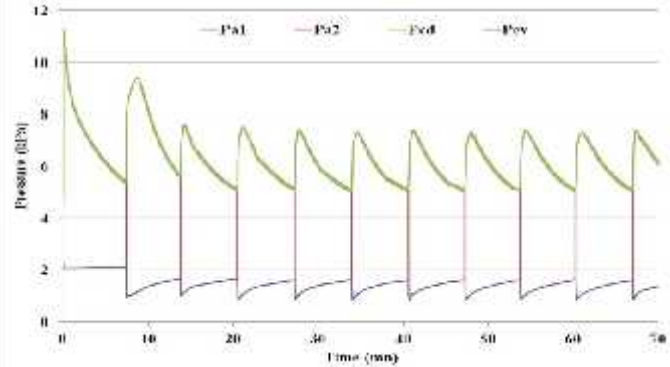
Figure 11 Pressure dynamic behavior at the adsorbents, condenser, and evaporator (numerical values)
