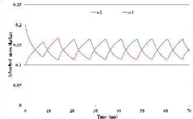
Figure 13 Adsorbed mass of water at the adsorbent beds (numerical values)
