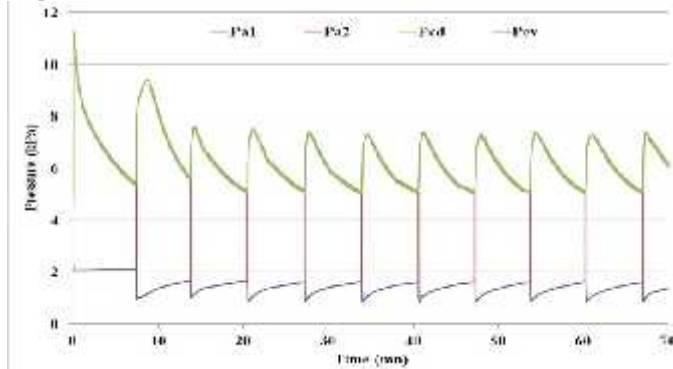
Figure 11 Pressure dynamic behavior at the adsorbent beds, condenser, and evaporator (numerical values)
