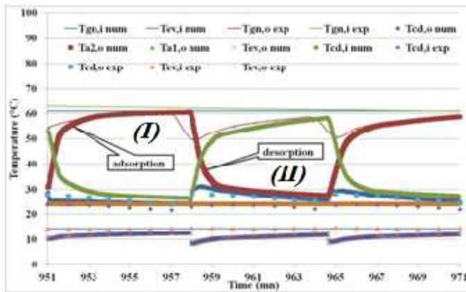
Figure 10 Temperatures profiles at the adsorbent beds, condenser, and evaporator (experimental and numerical)
