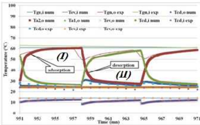
Figure 10 Temperatures profiles at the adsorbents, condenser, and evaporator (experimental and numerical)
