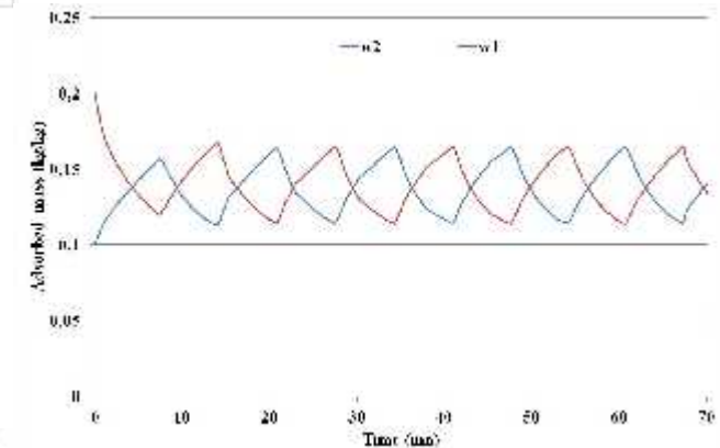
Figure 13 Adsorbed mass of water at the adsorbent beds (numerical values)
