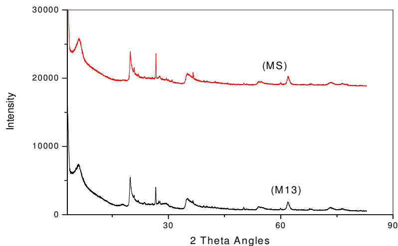
Figure 2. X-ray diffraction patterns of curves Maghnite (M13) and APTES–Maghnite (MS)
