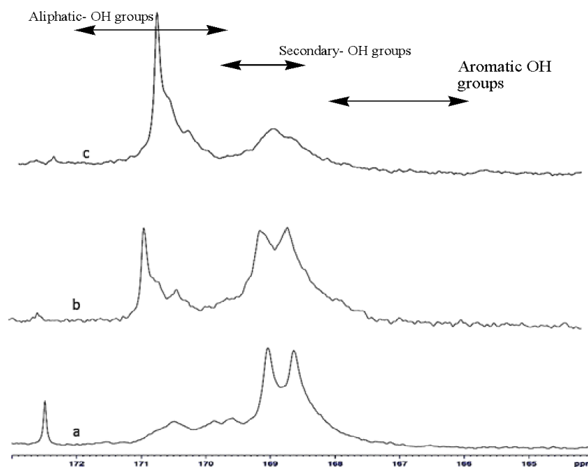
Fig. 3. 13 C NMR spectra of expanded hydroxyl region of (a) acetylated KL, (b) acetylated liquefied KL with PEG/ GLY, and (c) acetylated liquefied OPEFB with PEG/ GLY
