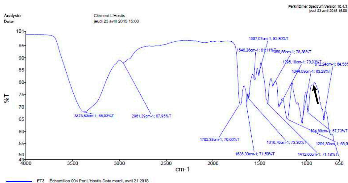
Figure 2. FTIR spectrum of the ET3 tannin epoxy acrylic resin sample.
