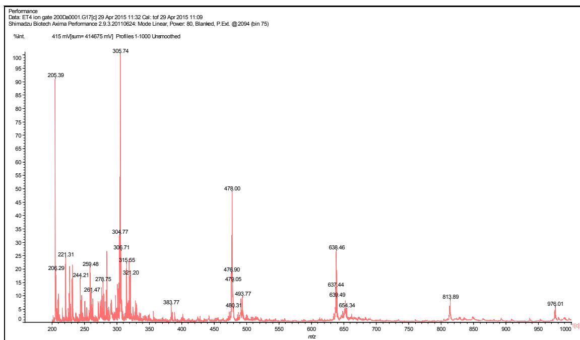
Figure 6. MALDI-TOF spectrum of the ET3 sample of tannin epoxy acrylate resin.
