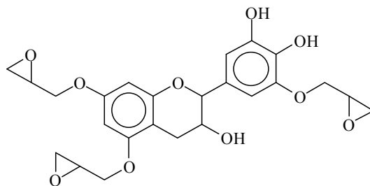
Scheme 3. Most probable structure of the 476 Da MALDI peak.
