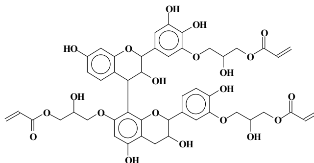
Scheme 8. Chemical structure describing the 976 Da MALDI peak.
