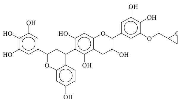
Scheme 5. Robinetinidin-galocatechin dimer with one epoxy group equally representing the 654 Da MALDI peak.
