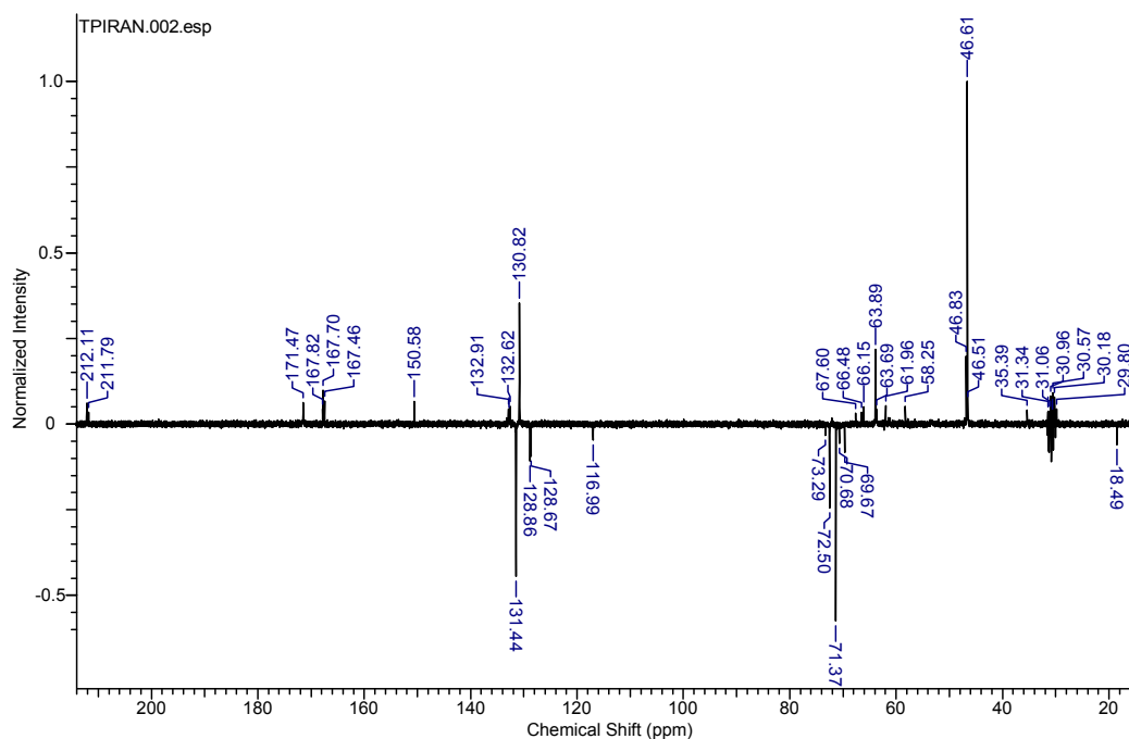
Figure 3. ^{13}\text{C} -NMR spectrum of the ET3 tannin epoxy acrylate resin.
