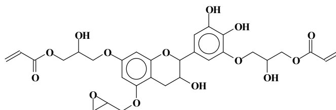
Scheme 6. Chemical structure describing the 638–639 Da MALDI peak.
