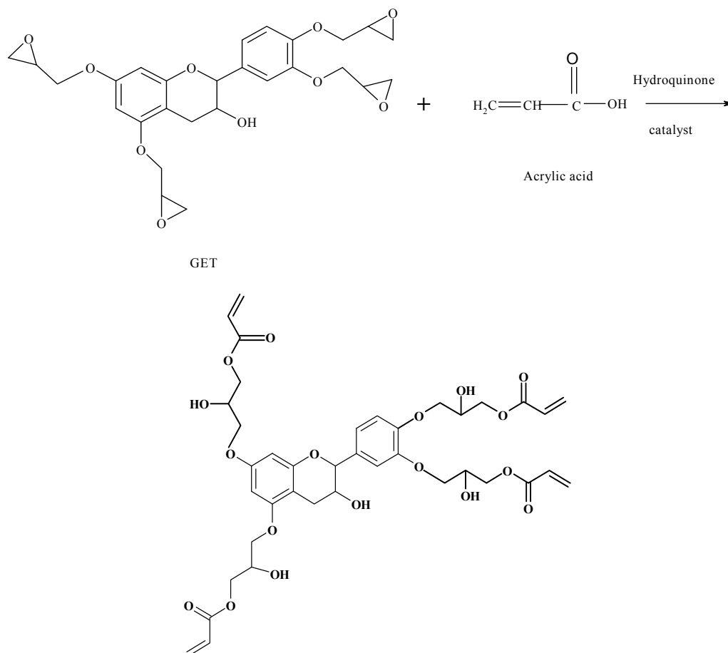
Figure 5. Reaction scheme of glycidylation of the tannin with acrylic acid (tannin-based epoxy acrylate).
