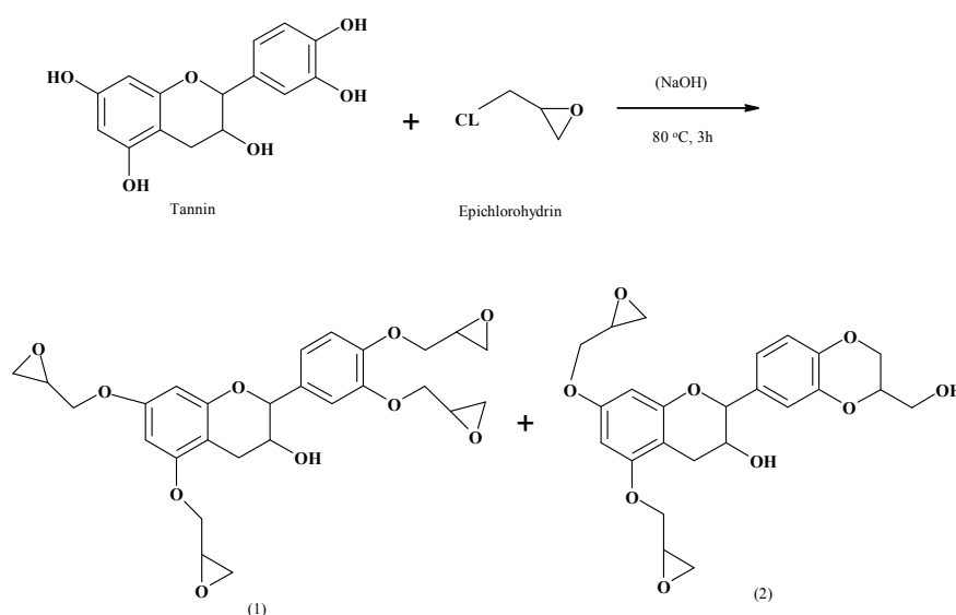
Figure 4. Reaction scheme for the epoxidation of tannin. Formation of epoxy groups on different sites of tannin's flavonoid units.
