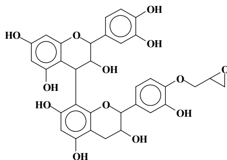
Scheme 4. Catechin dimer with one epoxy group representing the 654 Da MALDI peak.
