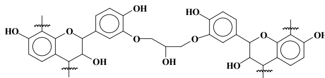
Scheme 2. Epoxy tannin oligomers as previously identified.
