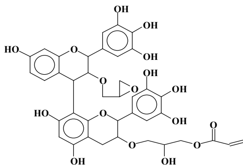
Scheme 7. Chemical structure describing the 813 Da MALDI peak.
