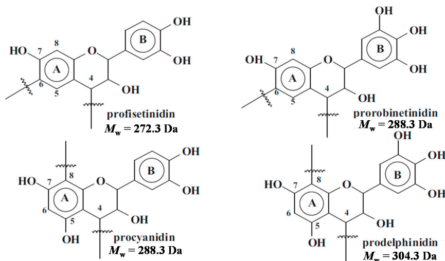
Figure 1. The four main structures in commercial flavonoid tannins.
