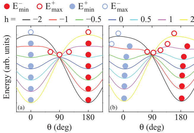
FIG. 2. (Color online) Evolution of the energy landscape of a macrospin system as a function of the angle \theta between the perpendicular axis and the macrospin for different reduced applied magnetic fields ( h = \frac{H}{H_k} ) (a) with the uniaxial symmetry ( \lambda = 0^\circ ) and (b) when it has been broken ( \lambda = 5^\circ ). The circles highlight the evolution of the equilibrium positions and permit to define the two energy minima E_{\min}^- and E_{\min}^+ and the two energy maxima E_{\max}^- and E_{\max}^+ .
