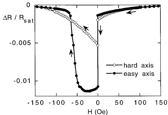
FIG. 2. Magnetoresistance effect \Delta R/R_{\text{sat}} , where R_{\text{sat}} = R(H_{\text{max}} = 200 \text{ Oe}) , measured at 4.2 K with a field applied along the easy and hard axis for a \text{Co}_{65}\text{Fe}_{35}/\text{Ag}/(\text{Co}_{65}\text{Fe}_{35})_{50}\text{Gd}_{50} (100 Å/80 Å/100 Å) trilayer (glass substrate).
