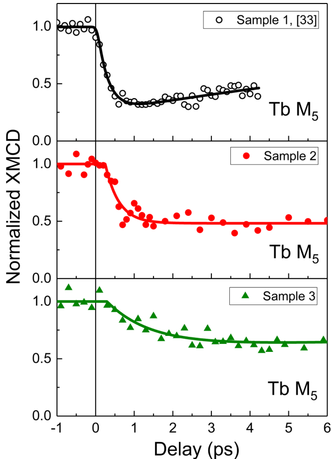
FIG. 3. Transient normalized XMCD at the Tb M_5 edge for samples 1, 2, and 3. For samples 2 and 3, the solid lines are fits in the framework of the three-temperature model. For sample 1, which is used to set the temporal overlap in this experiment, we superpose the data (open circles) and the fit of our previous Tb M_5 dynamics taken in the same experimental configuration [33]. The different sample configurations (samples 1, 2, and 3) show the respective characteristic demagnetization times of \tau = 0.28 \pm 0.03 ps, 0.35 \pm 0.1 ps, and 1.2 \pm 0.4 ps. The data in Fig. 3 (top panel) are reproduced with the authorization of the American Physical Society.
