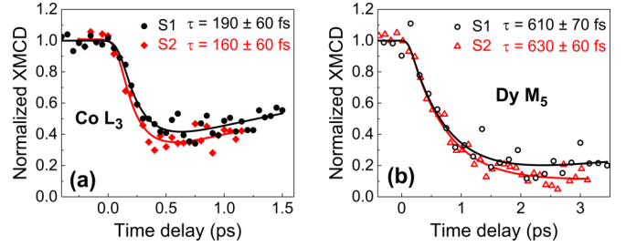
FIG. 6. Transient normalized XMCD at the Co L_3 (a) and Dy M_5 (b) edges for the S1 (black symbols) and the S2 (red symbols) alloys as a function of the delay. The solid lines are fits to the data by a double exponential convoluted by a Gaussian function. The laser fluence was 7 \text{ mJ/cm}^2 .
