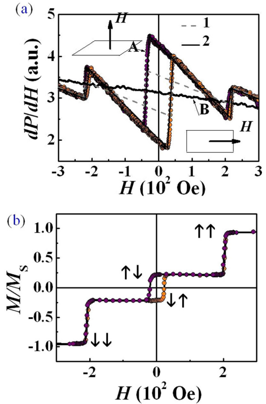
FIG. 3. (a) Field dependences of the first derivation of microwave absorption dP/dH(H) in the bilayer (sample II) for the upward and backward magnetic field H sweeping at temperature T=300 K, for two different orientations of the magnetic field with respect to the sample plane: configuration A corresponds to 0^\circ and configuration B corresponds to 90^\circ . Modelling of the hysteresis loop of the dP/dH(H) with no interlayer TMR is shown by dashed line 1. Solid line 2 is theoretical hysteresis loop dP/dH(H) assuming contribution of the TMR. (b) Magnetic hysteresis loops recorded in the SQUID magnetometer for the double layer (sample II) at T=300 K. Arrows show magnetization directions of the bottom layer (left arrow) and upper layer (right arrow).
