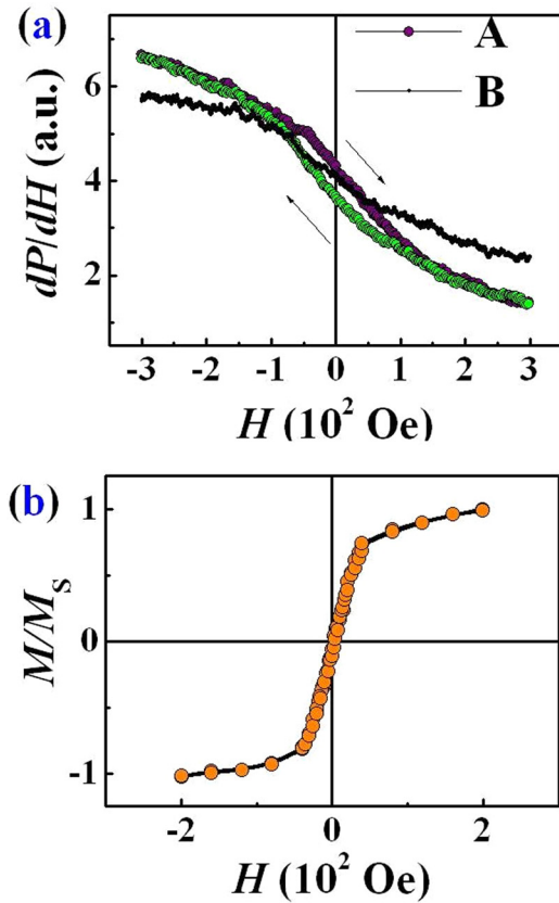
FIG. 2. (a) Field dependences of the first derivation of microwave absorption dP/dH(H) in the single layer (sample I) for the upward and backward magnetic field H sweeping at temperature T = 300 K, for two different orientations of the magnetic field with respect to the sample plane: configuration A corresponds to 0^\circ and configuration B corresponds to 90^\circ . (b) Magnetic hysteresis loops recorded in a SQUID magnetometer for single layer (sample I) and at T = 300 K.
