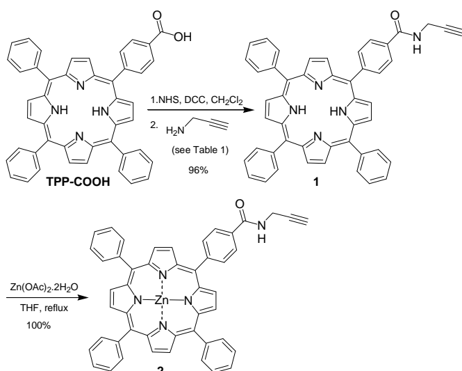
Scheme 1. Synthesis of alkyne-functionalized ZnTPP 2
