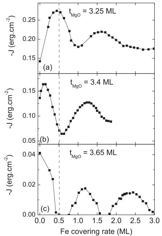
FIG. 5. Antiferromagnetic bilinear coupling constant measured at room temperature by Kerr magnetometry as a function of the Fe covering rate of the Fe buffer for three MgO spacer thicknesses: (a) 3.25 ML; (b) 3.4 ML; (c) 3.65 ML. The stack of the sample is Fe (50 nm)/MgO ( t ML)/Fe (5 nm).
