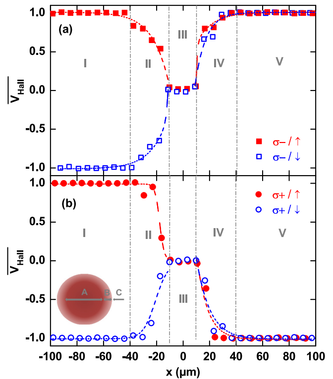
FIG. 2. Normalized Hall voltage \overline{V}_{Hall} as a function of the position of the beam x swept where (a) corresponds to left-handed circular polarization ( \sigma- ) and (b) to right-handed circular polarization ( \sigma+ ). The values 1 and -1 of the \overline{V}_{Hall} are the saturation of magnetization values. The laser beam is swept over the whole x axis of Hall cross from position -100\ \mu\text{m} to 100\ \mu\text{m} , with a sweeping speed of 40\ \mu\text{m}/\text{s} and a power of 0.95\ \text{mW} . The experiment is repeated for both positive and negative saturation of the magnetization. The dashed lines are guides to the eyes. Shown in the inset is the schematic presentation of the different areas of the laser spot: "A" where multiple domains are obtained (approximately 80\ \mu\text{m} diameter); "B" where AO-HDS is obtained ( 2-3\ \mu\text{m} size); "C" where no change of magnetization is induced.
