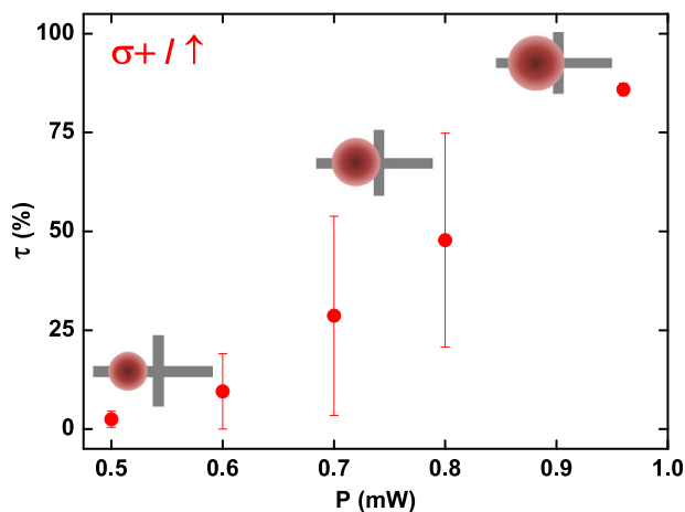
FIG. 4. Switching ratio \tau as a function of the laser power P for the static beam measurement. The center of the beam spot is kept fixed at a position approximately 40 \mu\text{m} from the Hall cross center. Shown in the inset is the schematic evolution of the diameter of the all-optical switching ring.
