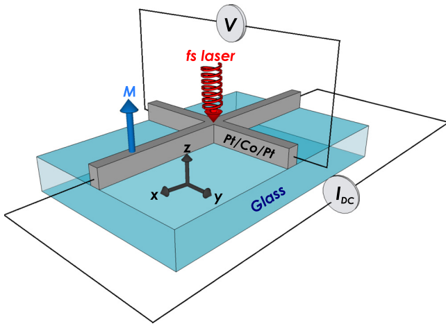
FIG. 1. Experimental set-up schematic: In a 5\ \mu\text{m} wide Hall cross of a ferromagnetic Pt/Co/Pt film showing perpendicular magnetization (z axis), a DC is injected along the x direction while the anomalous Hall voltage is measured along the y direction. The fs laser beam perpendicular to the film plane is swept along the x axis to perform the sweeping beam measurement, while for the static beam measurement; the laser spot is shined on the x axis at a fixed position about 40\ \mu\text{m} from the center of the Hall cross.
