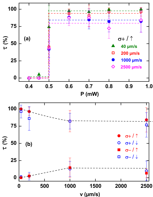
FIG. 3. (a) Switching ratio \tau as a function of the laser power P for different sweeping speeds. The initial saturation up with \sigma^+ sweeping is exemplarily shown. (b) Switching ratio \tau as a function of the swept beam's speed v with a power of 0.95 \text{ mW} for the four different combinations of circular polarization and initial saturation. The dashed lines are guides to the eyes.
