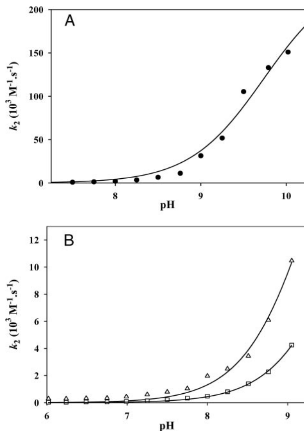
FIGURE 1. pH dependence of the second-order rate constant k_2 for the reaction of the thiol group with 2PDS of wild-type (●, panel A) and C51S (□, panel B) and C198S (Δ, panel B) MsrAs. Reaction kinetics were performed at 25 °C over a pH range of 5–9 or 10 in polybuffer B. The concentrations of enzymes and 2PDS were 6.2 and 310 \mu\text{M} , respectively. Values of k_{\text{obs}} were determined using nonlinear regression analysis, and second-order rate constants k_2 were fitted to Equation 2 (solid line) (see also “Experimental Procedures”). The plateau of the sigmoidal plot was not attained at the pH tested. Therefore, the pK_{\text{app}} values obtained by fitting could only be taken as estimates.
