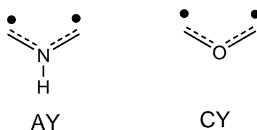
Scheme 1. Pseudodiradical structures of the simplest azomethine ylide (AY) and CY.
