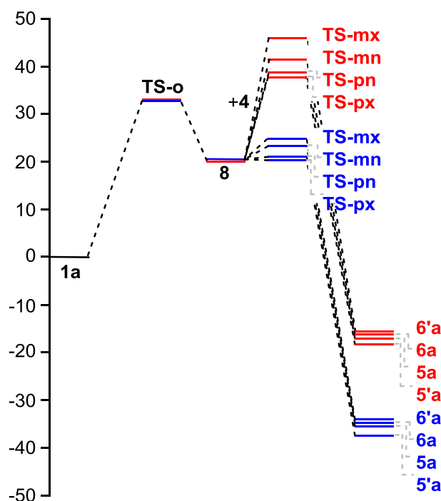
Figure 2. Enthalpy, in blue, and Gibbs free energy, in red, profiles (in kcal·mol -1 ) associated with the domino reaction between the oxirane 1a and 2-cyclopentenone ( 4 ) in toluene. Relative energies are given with respect to 1a + 4 .
