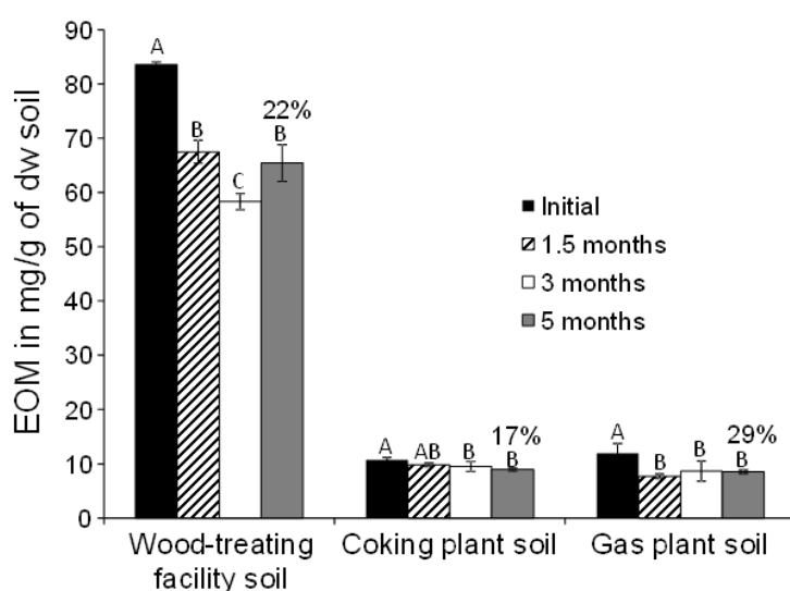
Figure 2: Extractable organic matter (EOM) of the initial soils and after 1.5, 3 and 5 months of microbial incubation (n=3; \pm SD). Percentages indicate the EOM decrease rate after 5 months of experiment. Letters indicate significant statistical differences (one-way Anova and Neuman-Keuls post-hoc test, p < 0.05 ) during time.
