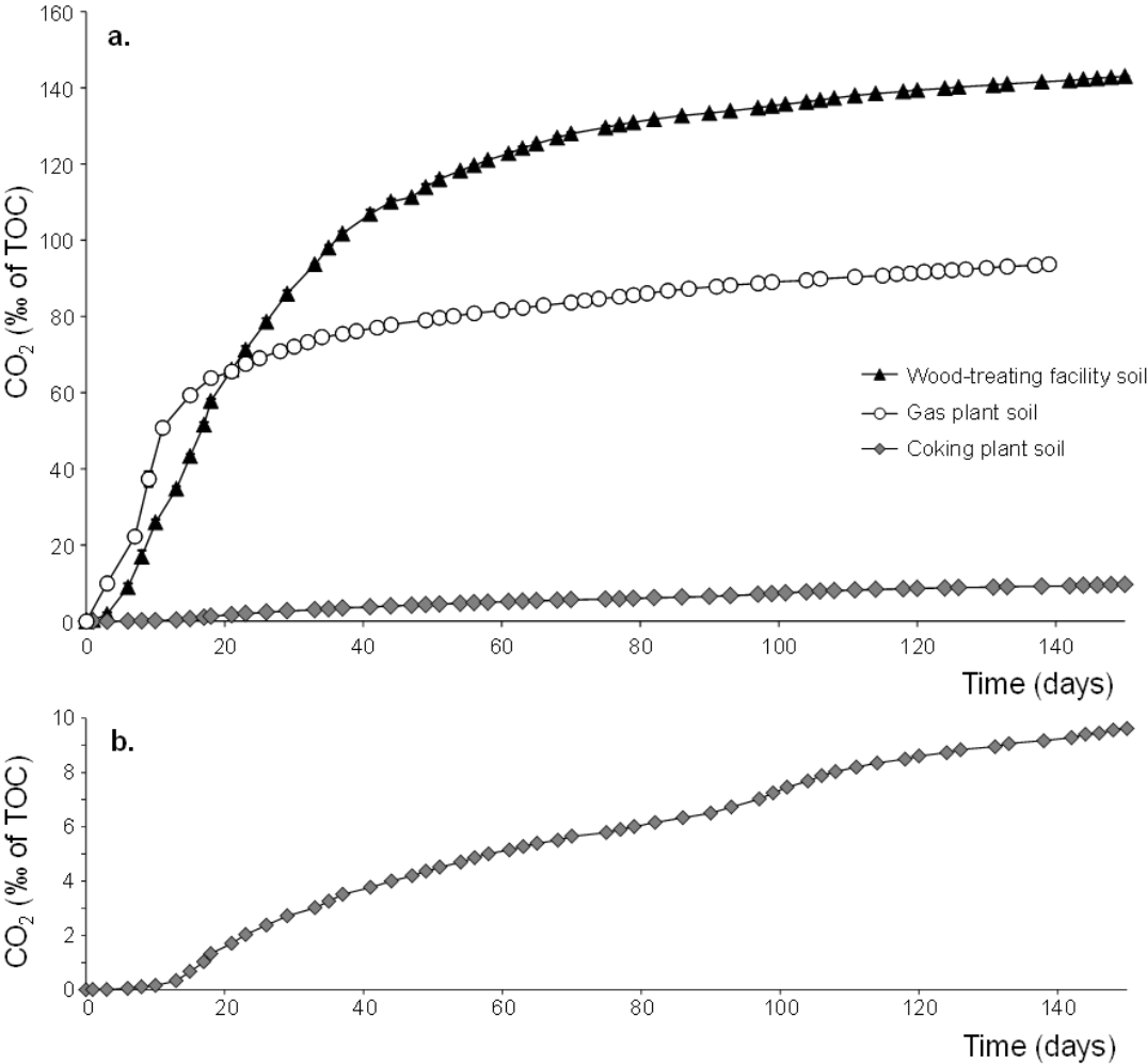
Figure 1: CO 2 released during the microbial incubation a) of the three soils (n=3 ± SD) and b) zoomed portion for the coking plant soil.
