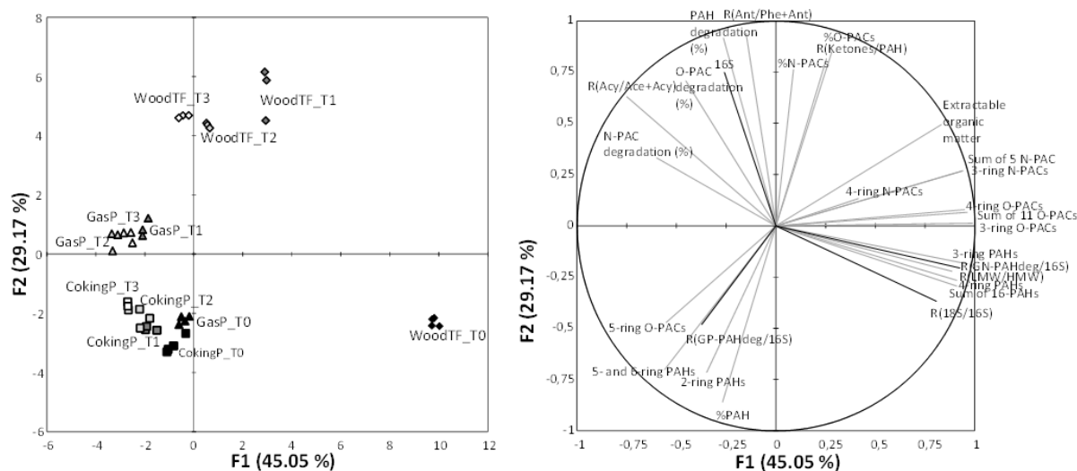
Figure 3: Principal component analysis (PCA) and correlation circle, based on organic and microbial parameters (grey and black vectors, respectively) for the three soils (wood-treating facility, WoodTF; coking plant, CokingP; and gas plant, GasP) at the four sampling times (T0, T1, T2 and T3). Abbreviations on the correlation circle correspond to R(LMW/HMW): ratio of low molecular weight over high molecular weight PAHs; R(ketones/PAH): ratio of ketones over 16 PAH content; R(Ant/Phe+Ant): ratio of anthracene over sum of phenanthrene and anthracene contents; R(Acy/Ace+Acy): ratio of acenaphthylene over sum of acenaphthene and acenaphthylene contents; %PAH, %O-PAC and %N-PAC: percentage of each class of compounds (sum = 100%); 16S: abundance of bacterial 16S rDNA genes; R(18S/16S), R(GN-PAH-deg/16S), R(GP-PAH-deg/16S): ratio of fungal 18S rDNA gene, and PAH-RHD \alpha from Gram negative and Gram positive bacteria over 16S rDNA gene abundance.
