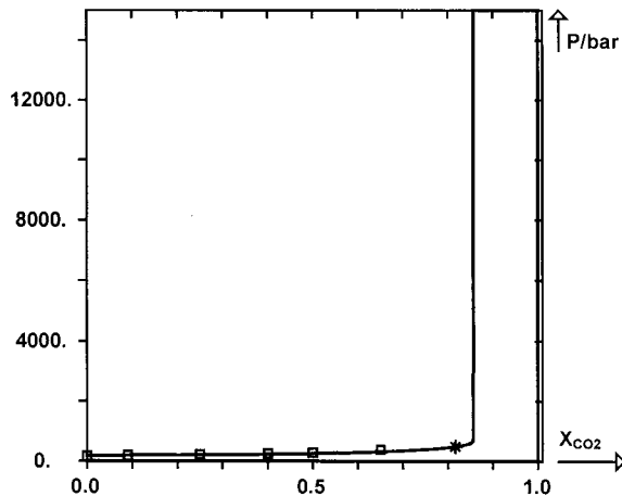
Figure 3. Swelling test performed on fluid F13 (pure \text{CO}_2 is injected): evolution of the saturation pressure versus quantity of injected gas. Experimental data points are shown as boxes. The continuous lines are the predicted values (the calculation becomes impossible as soon as x_{\text{CO}_2} becomes higher than 0.85).
