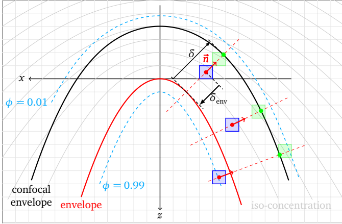
Fig. 3 Schematic illustration of the method used to compute the envelope propagation velocity, \tilde{V}_n , for all grid cells within the transition region of the indicator field: 0.01 < \phi < 0.99 (blue cells). The supersaturation \Omega_\delta needed for this is the supersaturation of the liquid in the corresponding green dots, i.e. at the intersection of the confocal envelope and the line of the envelope normal vector running through the center of the blue cell (red dot). \Omega_\delta is calculated by interpolation across the neighborhood of the green cell.
