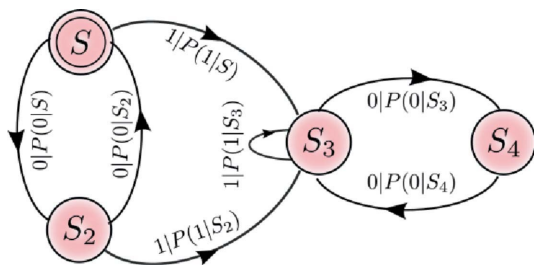
Figure 11 The mixed-state representation of the biased even process. The starting state is denoted by the double circle. Compare with Fig. 2 of Appendix A in Crutchfield et al. (2016).
