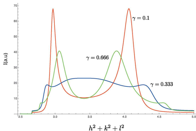
Figure 10 The behaviour of the {111} peaks for a powder diffraction pattern for different extrinsic faulting probability. The peaks not affected by faulting have been left out.
