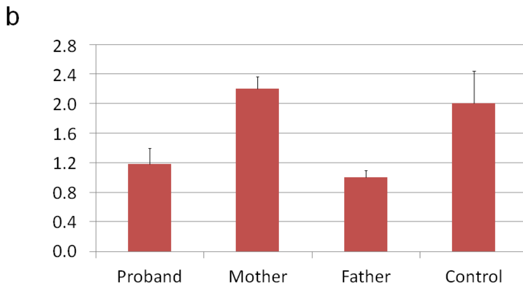
Supplementary Figure 2 Identification of a heterozygous deletion encompassing exon 4 of HCN1 in a female subject with ID and ASD, inherited from her asymptomatic father. (a) Cyto-12 SNP array (Illumina) profiles of the patient with HCN1 exon 4 deletion and details of the coding sequences included the deletion: the y axis indicates the B allele frequency (above) and the log R ratio (below), and the x axis indicates the position on chromosome 5. The deletion spans ~33 kb and theoretically leads to an in-frame deletion of 73 amino acids (p.Asn338_Lys410del) in the extracellular loop between the S5 and S6 domains containing the pore region. (b) Confirmation of the presence of the HCN1 heterozygous deletion in the proband and her father by quantitative PCR using primers located on exon 4 (forward: 5'-CCACCTGCTATGCCATGTTT-3'; reverse: 5'-ATACTGCCGCCTCGAAGsAAT-3'). RT-PCR experiments were performed using 10 ng of genomic DNA, 0.8 \mu M of each primer and 12.5 \mu l of SYBR Green PCR master mix (Applied Biosystems) in a total volume of 25 \mu l. RNase P (RNase P Control Assay, Applied Biosystems) was used as the reference amplicon. Each sample was run in triplicate on an ABI PRISM 7700 Detection System (Applied Biosystems), and three different experiments were used for final quantification. Relative ratios were calculated using the formula r = 2^{-\Delta\Delta C_t} with \Delta\Delta C_t = (C_{t \text{ mutation}} - C_{t \text{ RNaseP}})_{\text{ind tested}} - (C_{t \text{ mutation}} - C_{t \text{ RNaseP}})_{\text{ind ref}} .
