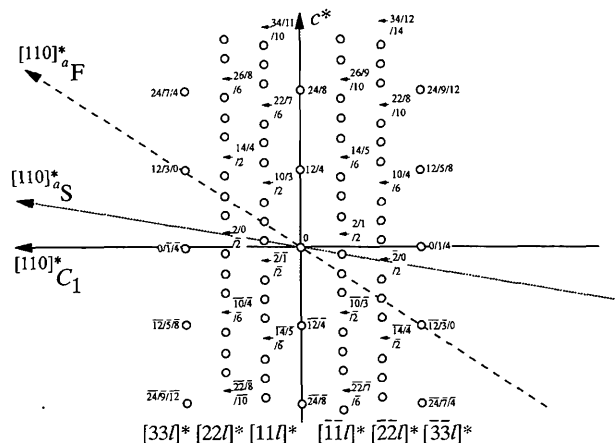
Fig. 5. (hhl) plane of 4M_3 mica lattice. For explanations, see Fig. 4. Along reciprocal-lattice rows, h = \pm 3 nodes corresponding to non-extinguished reflections (one out of four) are indexed, while along the other rows nodes corresponding to extinguished reflections (one out of four) are indexed.
