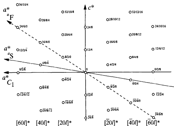
Fig. 4. (h0l) reciprocal-lattice plane of 4M_3 ( Z = 3531 ; RTW = \bar{2}\bar{2}\bar{2} ) mica lattice. The scale along c^* and a^* axes is not the same. Indexing: the three numbers represent the l index according to C_1 , {}^aS and {}^aF , respectively. For 00l , indexing according to both {}^aS and {}^aF coincides.
