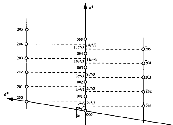
Fig. 2. Definition of Fixed-angle setting for multilayer polytypes. The (h0l) plane of the {}^a\mathbf{S} setting is shown, limited to h = 0, \pm 2 and l from 0 to 5. The projection of reciprocal-lattice nodes on the c^* axis never corresponds to an integral multiple of the period along c^* .
