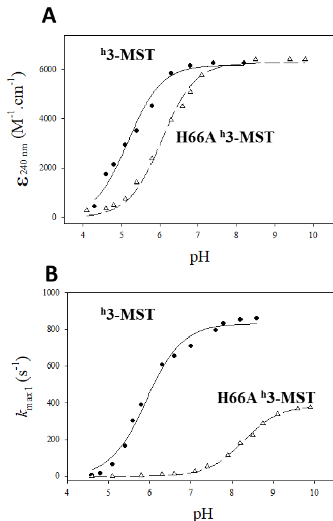
Figure 4: pH-dependence of the absorbance properties of the catalytic Cys237 (A) and of the rate-constant k_{\text{max}1} (B) for the wild-type ( \bullet ) and H66A ( \Delta ) h3-MSTs.
