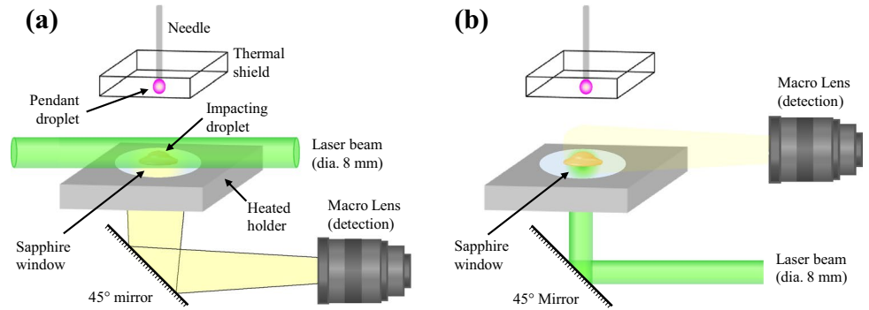
Fig. 7 The two optical configurations used to visualize the fluorescence emission of the impinging droplet a bottom view imaging, b side view imaging
