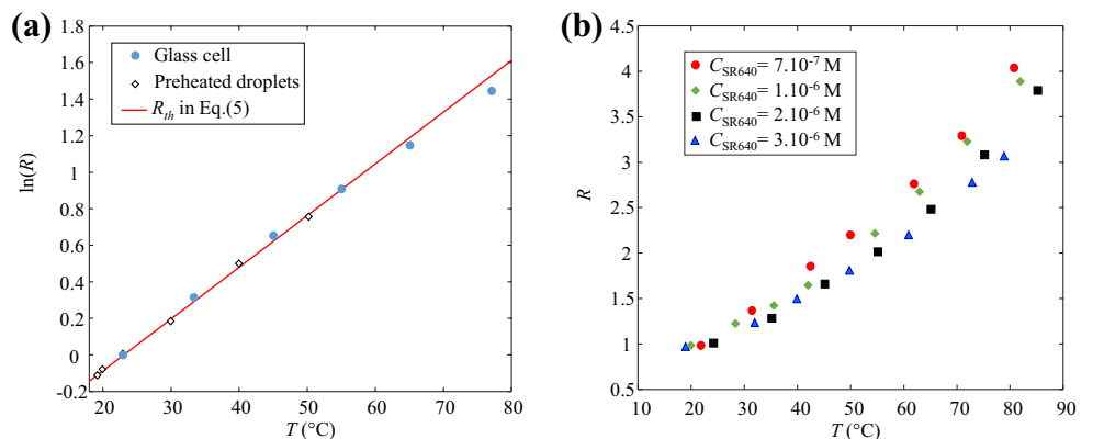
Fig. 8 Evolution of the fluorescence ratio R as a function of the temperature. R is normalized to be equal to 1 at 23^\circ\text{C} . a C_{\text{SR640}} = 7.10^{-7} \text{ M} and C_{\text{FL}} = 2.10^{-4} \text{ M} , b C_{\text{FL}} = 2.10^{-4} \text{ M}
