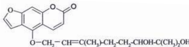
Figure 17 : structure du 6',7'-dihydroxybergamottine (39).
