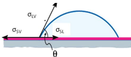
Figure 13: Angle de contact (Tadmor, 2004)
