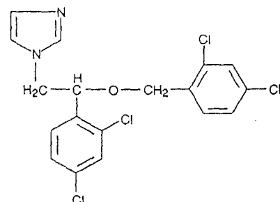
Miconazole
