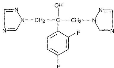
Fluconazole
