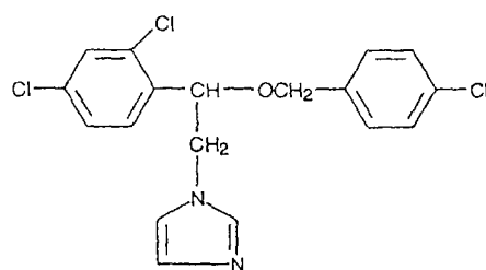
Econazole
