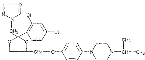
Terconazole
