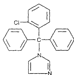
Clotrimazole
