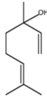
Figure 39 : Linalol
