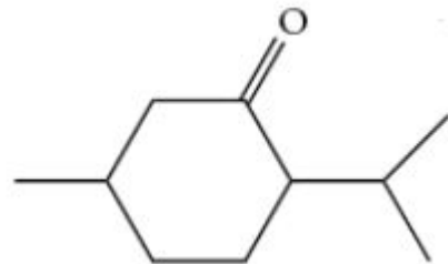
Figure 19 : Menthone
