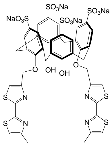
Figure 17 : Structure du C[4]S-BTZ
