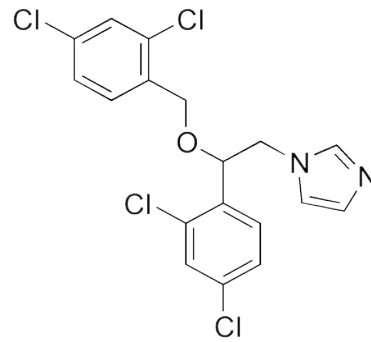
Miconazole
