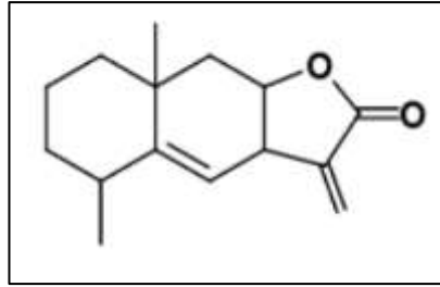
Figure 21 : Alandactone
