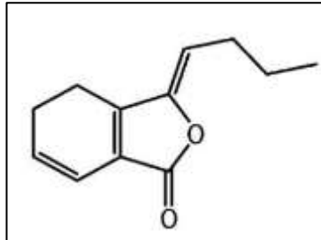
Figure 23 : Ligustilide
